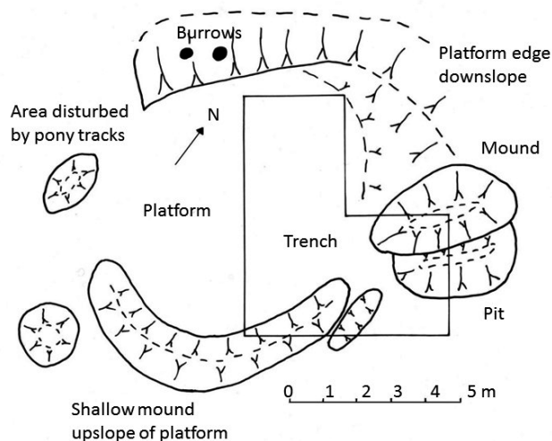
Fig. 4 Plan of the earthworks forming the platform site and the pit-and-mound feature, indicating the trench position. Drawing A. C. King
