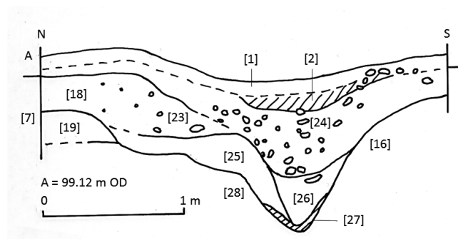
Fig. 8 Section drawing of the east side of the cut through the pit-and-mound feature. Drawing A. C. King
